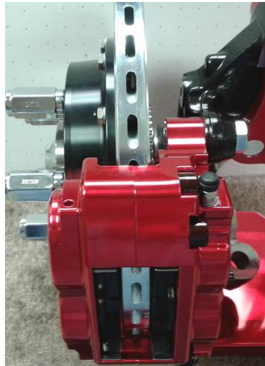
Figure 2: Caliper installed (side view)
